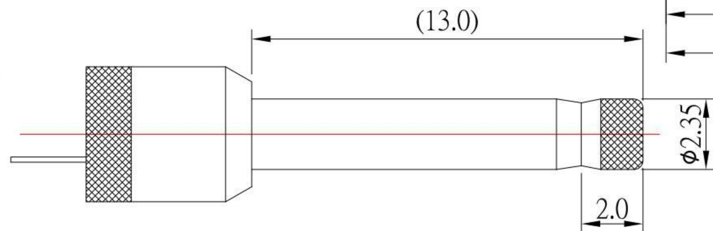
RECOMMENDED PLUG
