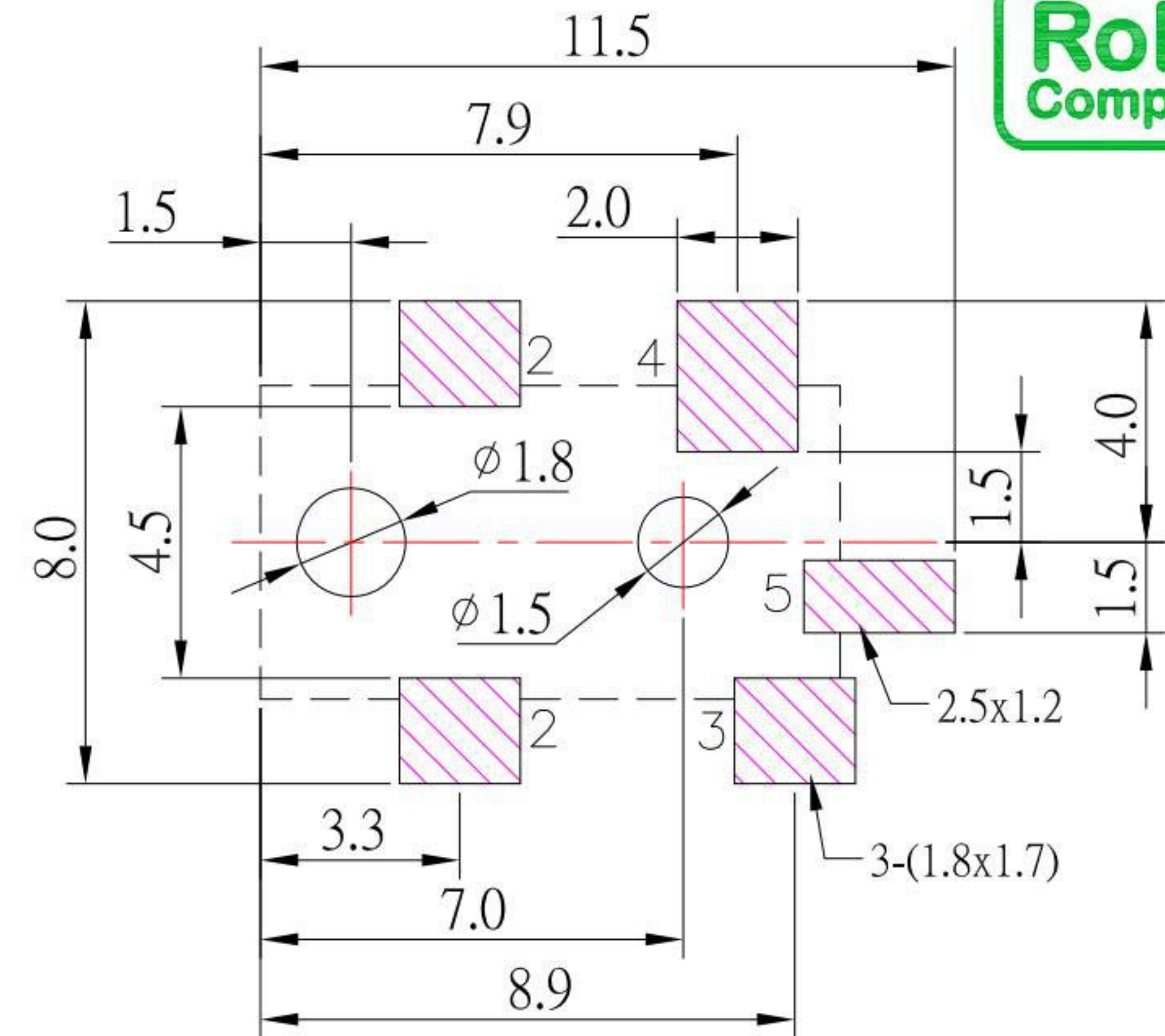
P.C.B. LAYOUT TOP VIEW
