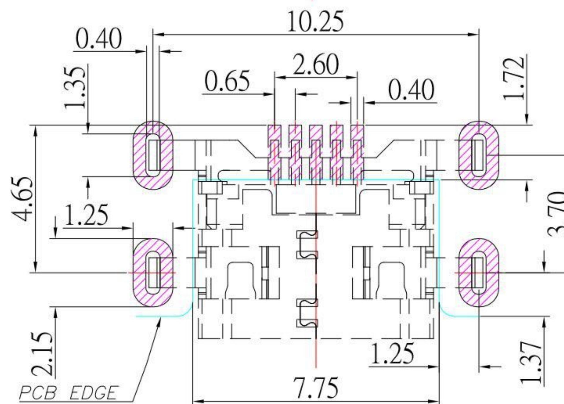
P.C.B LAYOUT MOUNTING PATTEN
