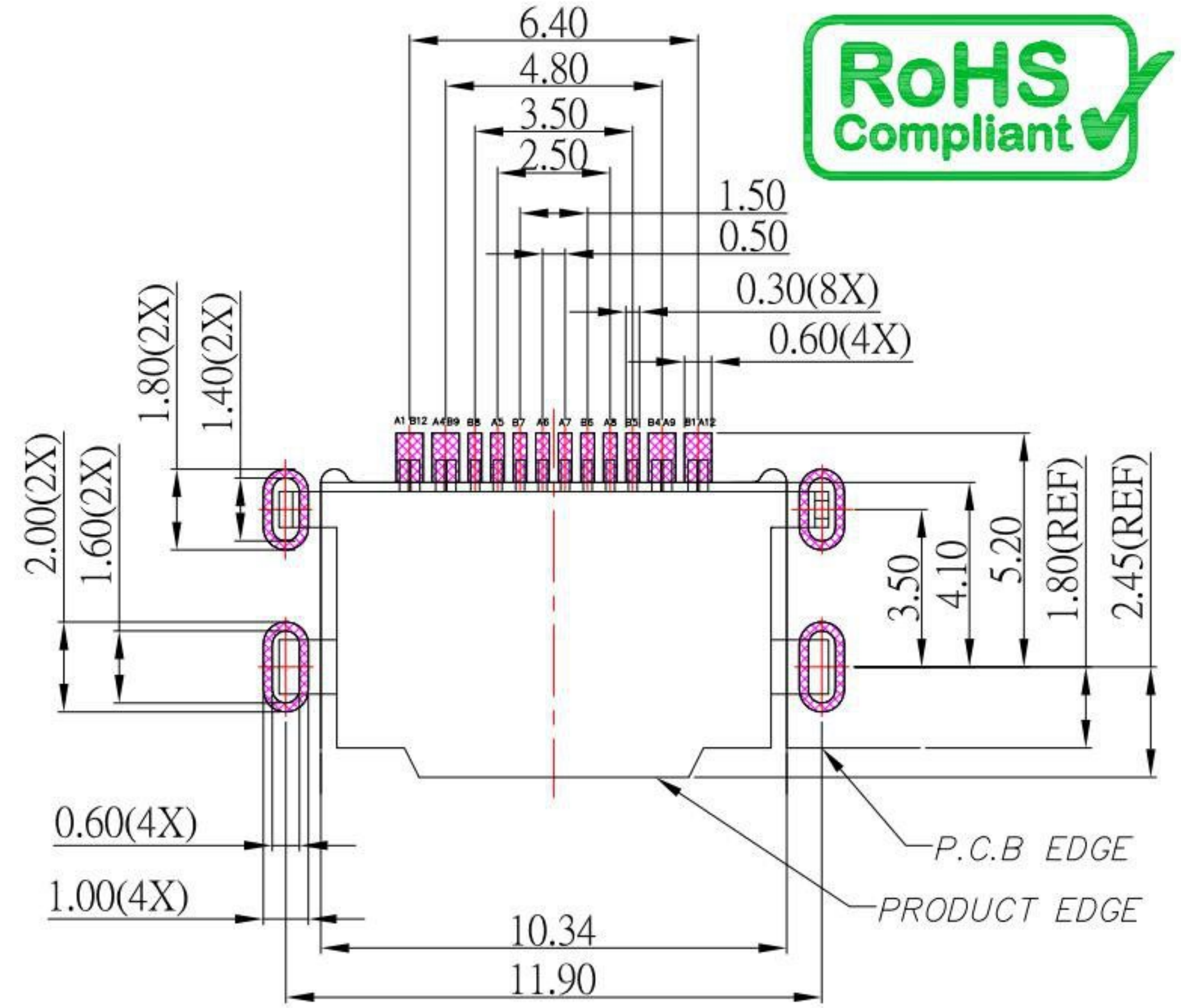
RECOMMENDED P.C.B. LAYOUT
