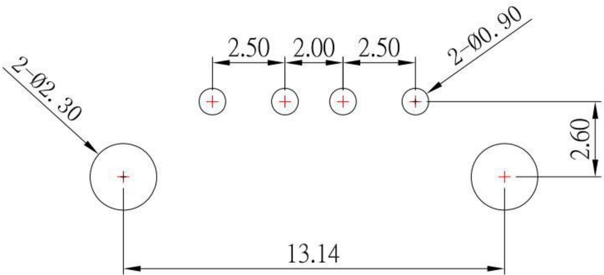
P.C.B LAYOUT MOUNTING PATTERN
