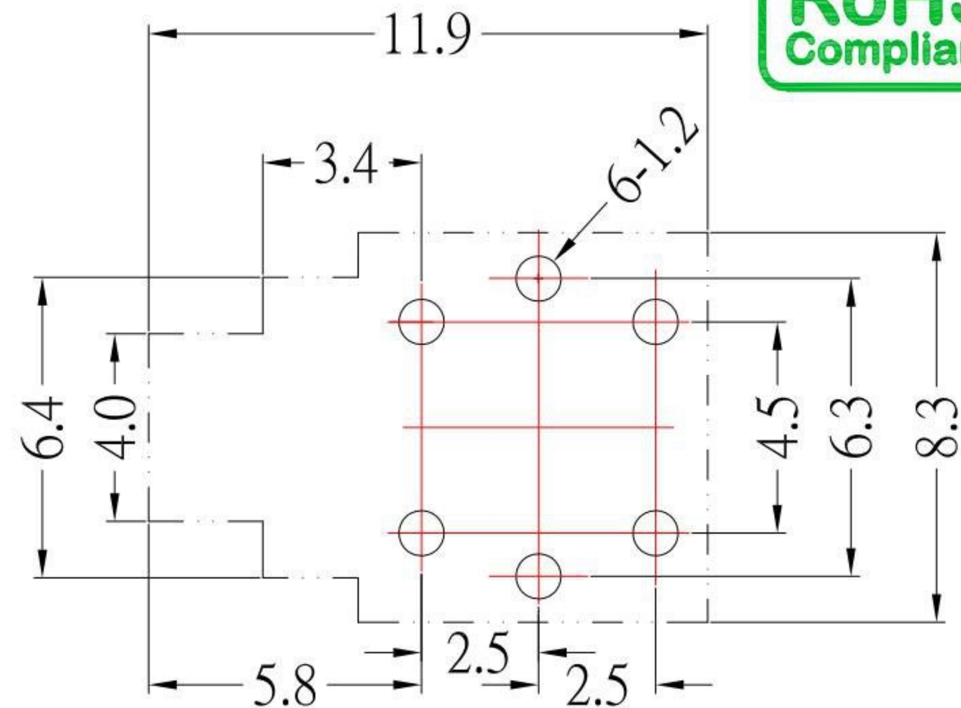
P.C.B LAYOUT BOTTOM VIEW
