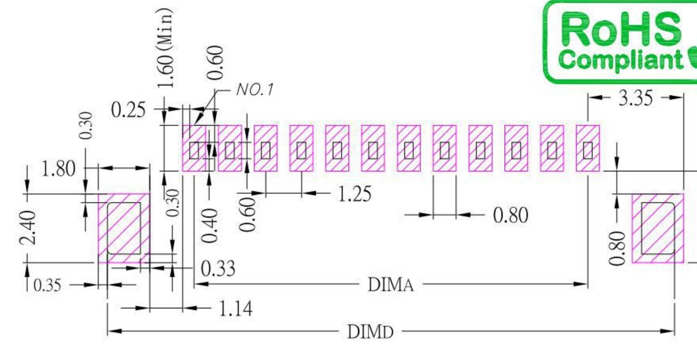
P.C.B LAYOUT MOUNTING PATTERN
